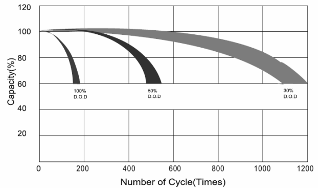
Cyclic Life Curve
